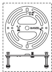
A Crossbar Assembly x 1
