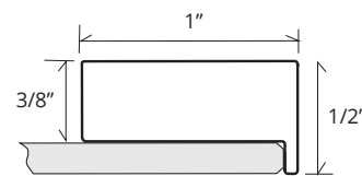
Section view - LEXINGTON FRAME
